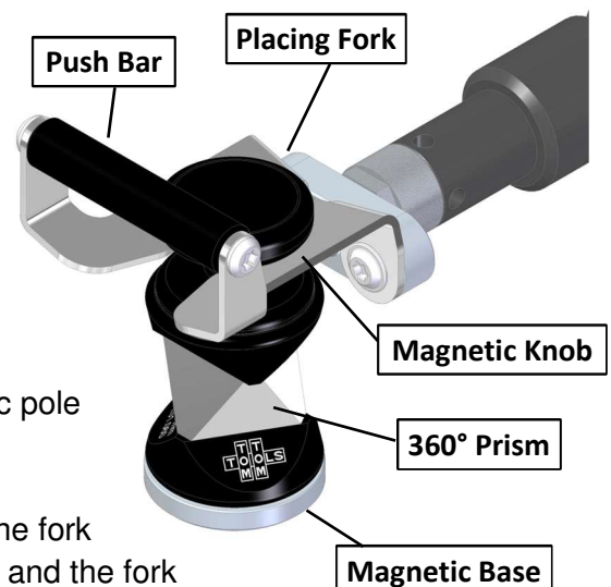
Fig.9.5.1 “360° Prism” on Placing Fork
