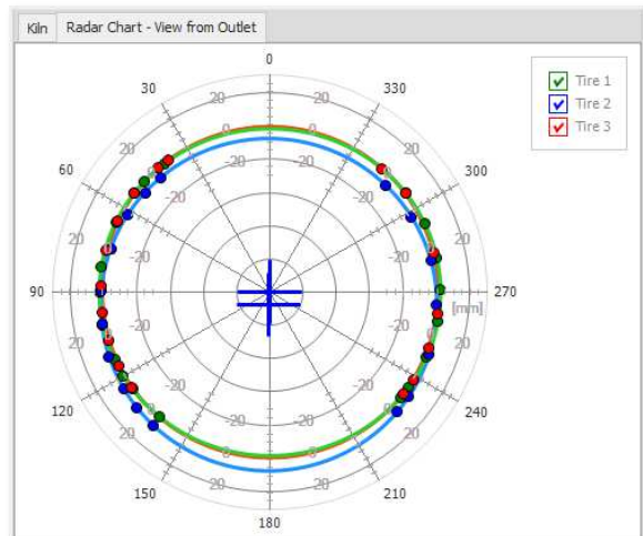
Fig.8.3.3 Radar Chart (where tire 1 and 3 are anchors)
