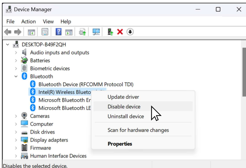
Fig.5.2.1 Device Manager
